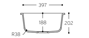
CROSS-SECTION
