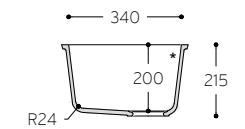
CROSS-SECTION
