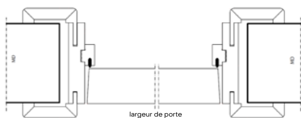
Coupe horizontale chambranle WoodFlex
