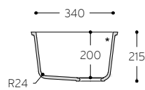
CROSS-SECTION
