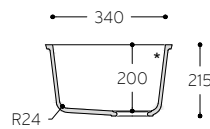
CROSS-SECTION
