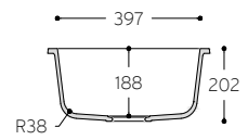
CROSS-SECTION
