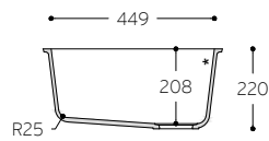
CROSS-SECTION
