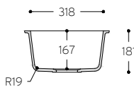
CROSS-SECTION
